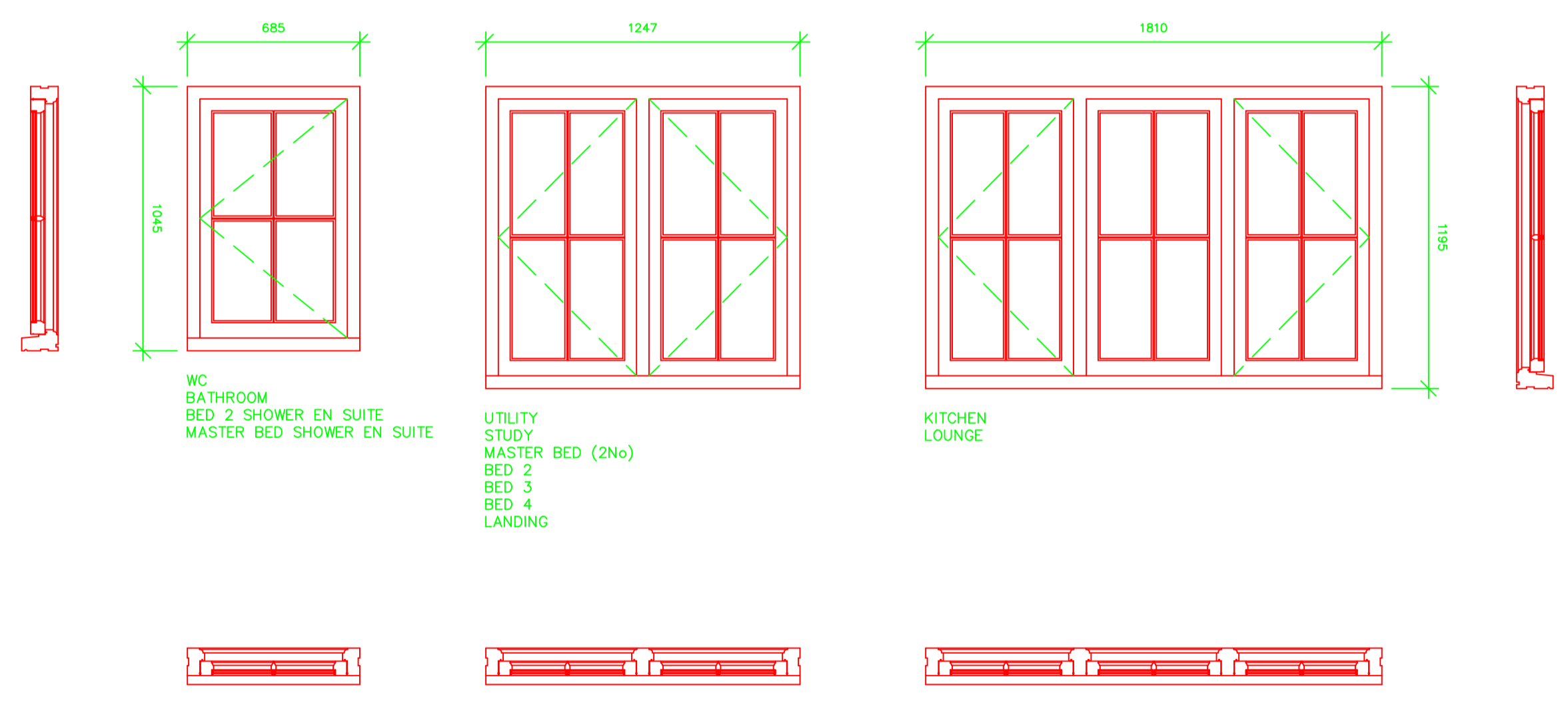
WINDOW JOINERY PLANS, SECTIONS + ELEVATIONS SCALE 1/20
